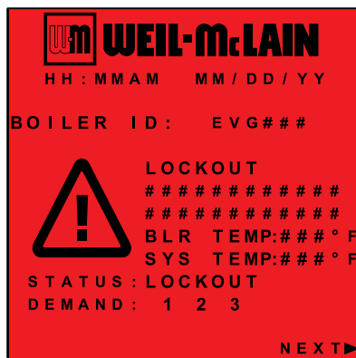
Figure 7 Evergreen™ boiler control display LOCKOUT SCREEN — screen turns red when boiler locks out — highlight and select MANUAL RESET to reset boiler as shown below.
