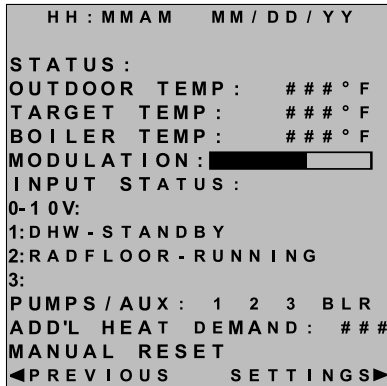
Figure 8 Evergreen™ boiler control display USER Menu — (set date and time, reset faults).
