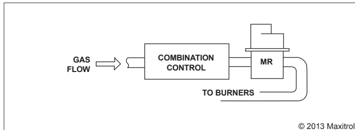
Figure 9 : If full combination control is used, install MR valve downstream. Adjust regulator in combination control 2 or 3 turns to compensate for pressure drop at MR valve.
