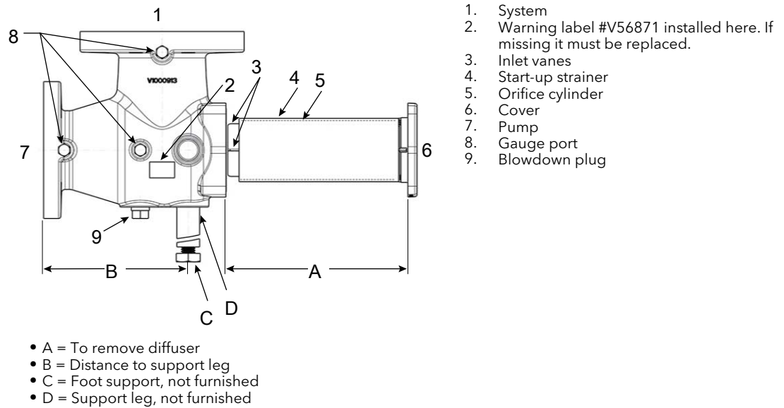
Figure 1: Working pressure 175 PSI (1207 KPa), 121°C (250°F)
