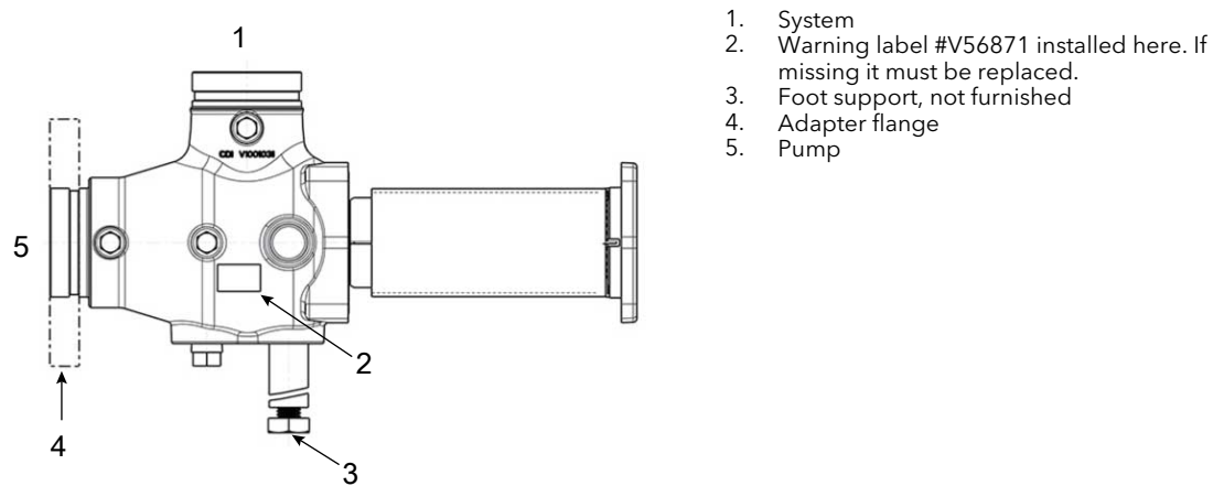
Figure 2: Working pressure 300 PSI (2069 KPa), 121°C (250°F)
